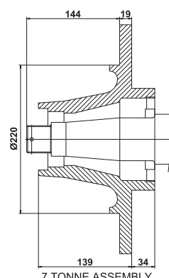
7 TONNE ASSEMBLY
