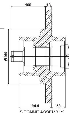
5 TONNE ASSEMBLY
