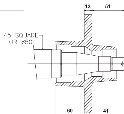
SLIMLINE 1.25 TONNE ASSEMBLY SMALL OR LARGE FLANGE HUB
