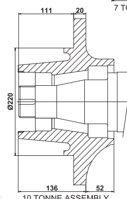
10 TONNE ASSEMBLY
